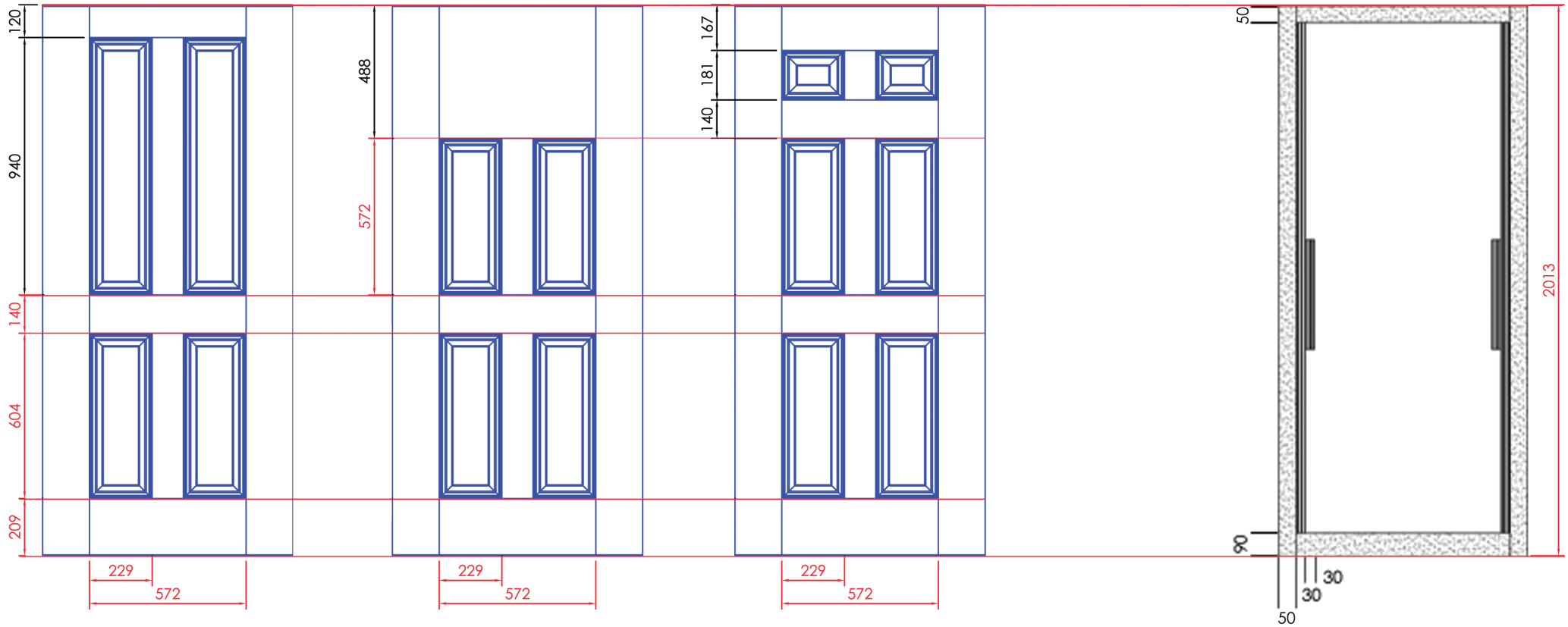
Recommended Routing Details (mm)
